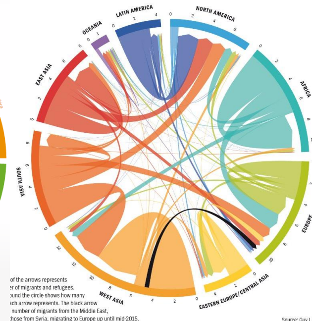
Migrant flows between regions of the world 2010–2015
